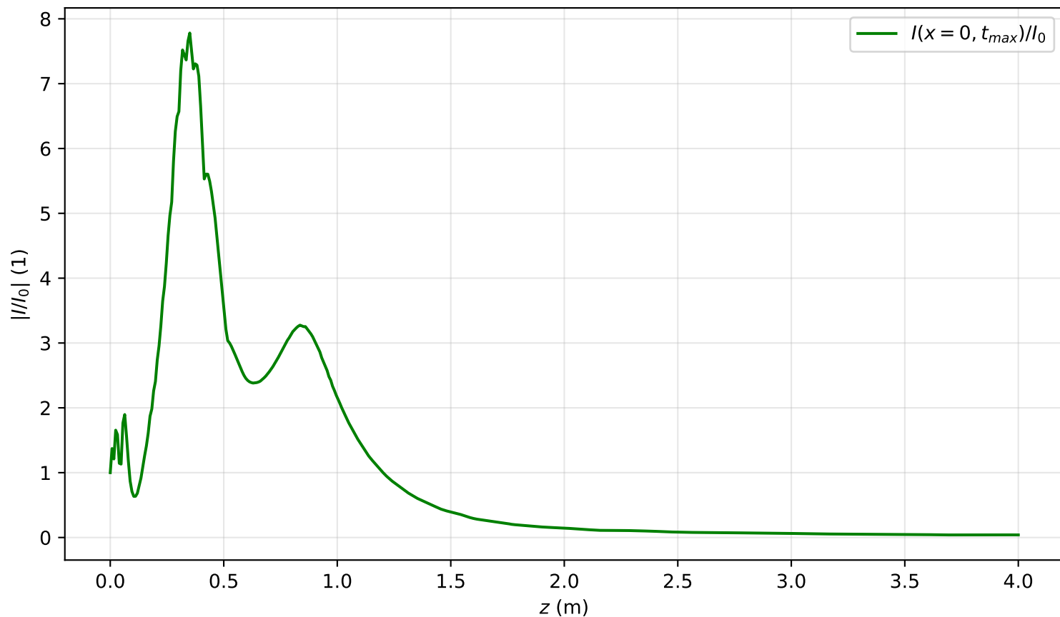
I(x=0, t_{max}, z)/I_0 , Pin=4.3Pcr
